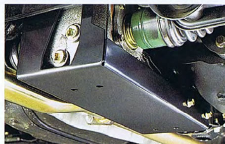
36 Differential protector B031SSA000 W Helps protect rear differential from rocks and logs.
