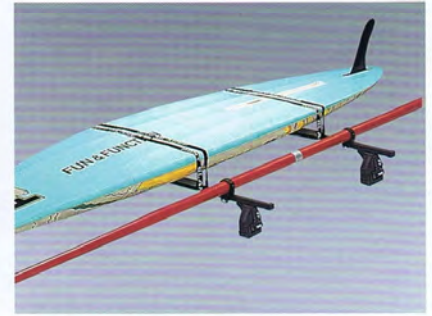
37. Sailboard attachment
